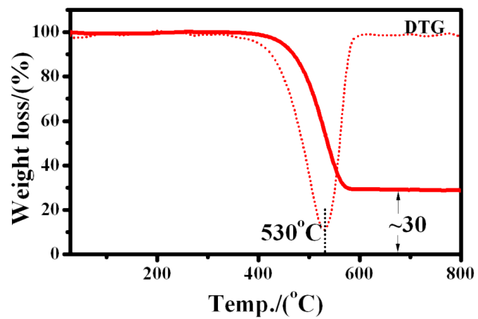
Figure S2 TG curve for the porous FeF 2 -CMK-3 hybrid composite recording at ramp rate of 10 °min -1 from room temperature to 800 °C.
