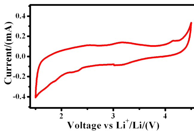
Figure S1 Typical cyclic voltammogram curve for the FeF 2 -CMK-3 hybrid scanning at 0.2 mVs -1 in a voltage window of 1.5-4.5 V.
