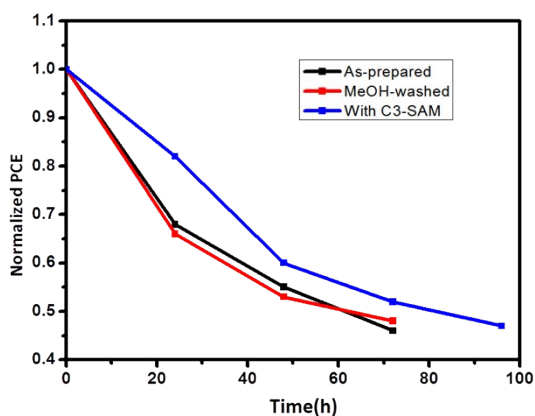
Fig. S1 Normalized PCE values as a function of aging time of devices based on different PEDOT:PSS substrates. PCE values are averages of 8 devices. The devices were stored in darkness in air with controlled relative humidity of 25%.
