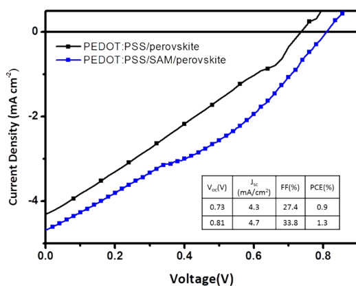
Fig. S2 Best J-V curves of full roll-to-roll fabricated devices. Forward bias to short-circuit voltage sweep was conducted from -0.1 to 1.0 V with voltage steps of 5 mV. The Ag electrode was screen-printed.
