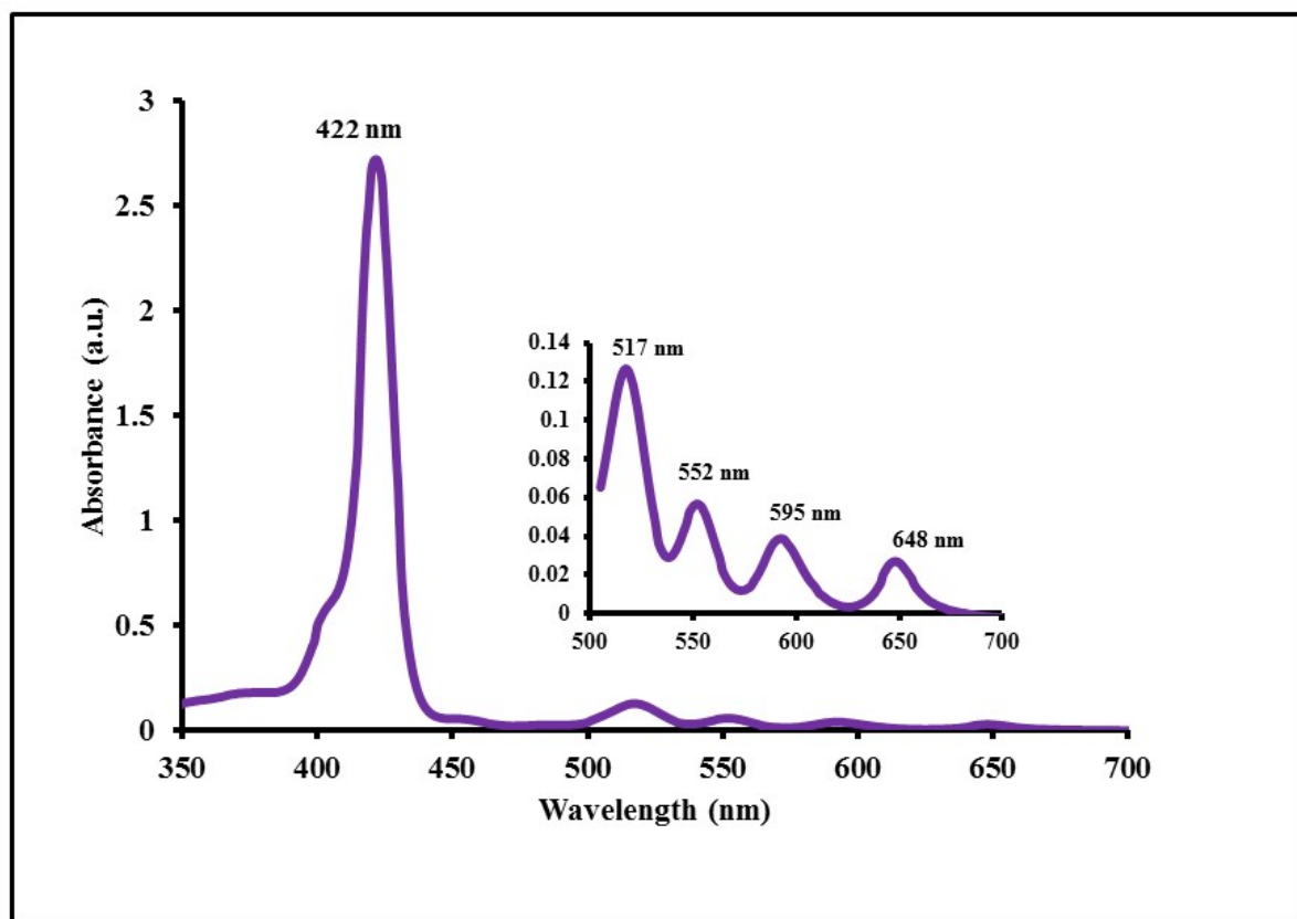
Figure S2. UV-Vis spectra (CH 3 Cl) of of meso-tetra (4-metoxyphenyl) porphyrin ( H 2 TCPP)
