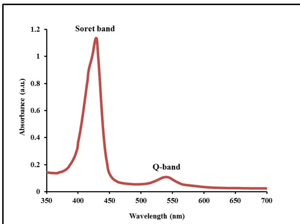
Figure S4. UV-Vis spectra (THF) of of Cobalt(II) meso-tetra (4-carboxyphenyl) porphyrin (Co-TCPP)
