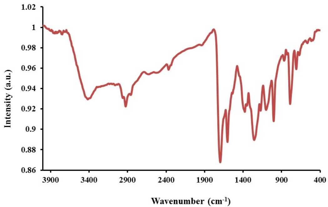
Figure S3. FT IR spectram (KBr) of Cobalt(II) meso-tetra (4-carboxyphenyl) porphyrin (Co-TCPP)
