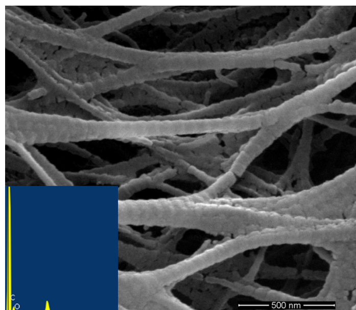
Figure S1. SEM image of the dentin surface after being demineralized with 37% phosphoric acid for 2 min. Energy disperse spectrum (EDS) (Insets) showed that there were no Ca and P elements on the demineralized surface.
