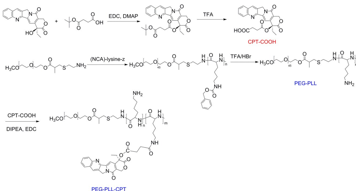
Supporting Scheme 1. The synthesis of the control CPT-drug conjugate PEG 45 -PLL 25 -CPT 6 .
