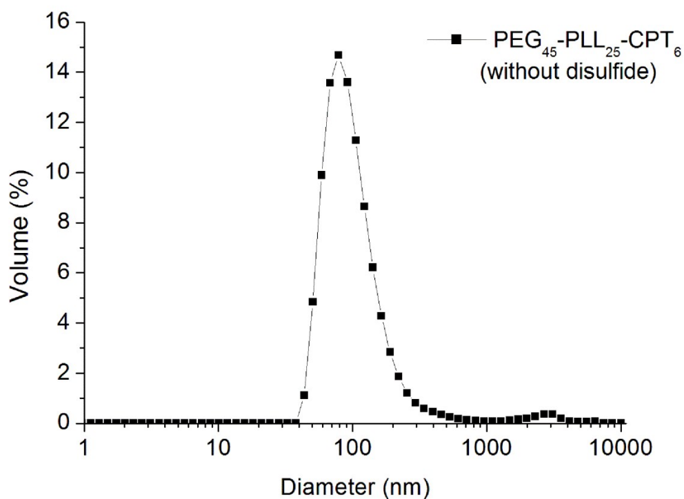
Supporting Figure 1. Micelle sizes measured by dynamic light scattering of PEG 45 -PLL 25 -CPT 6 (control CPT-nanoparticle, without disulfide bond).
