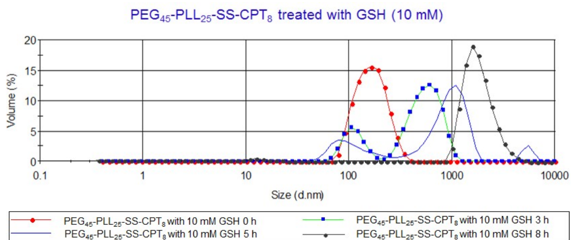
Supporting Figure 2. Micelle size change measured by dynamic light scattering of PEG 45 -PLL 25 -SS-CPT 8 after treated with GSH (10 mM).
