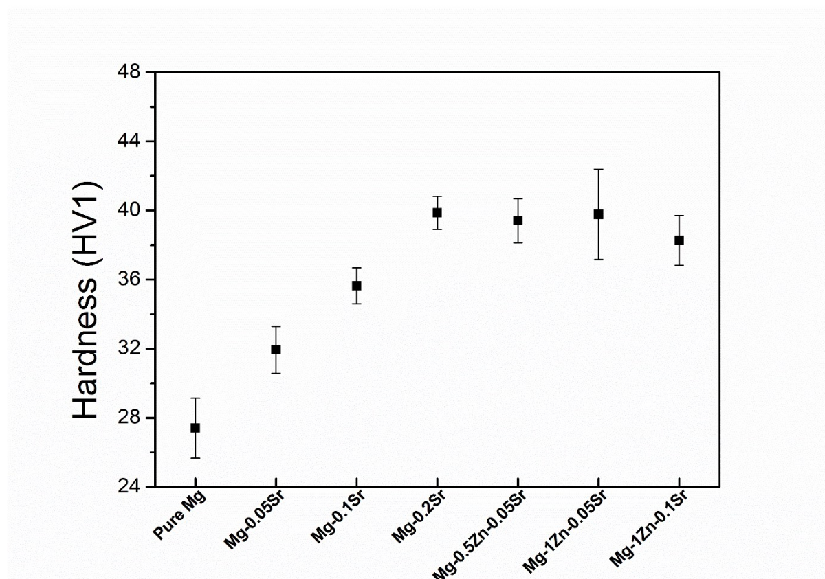
Figure 1# Microhardness of Mg alloys
