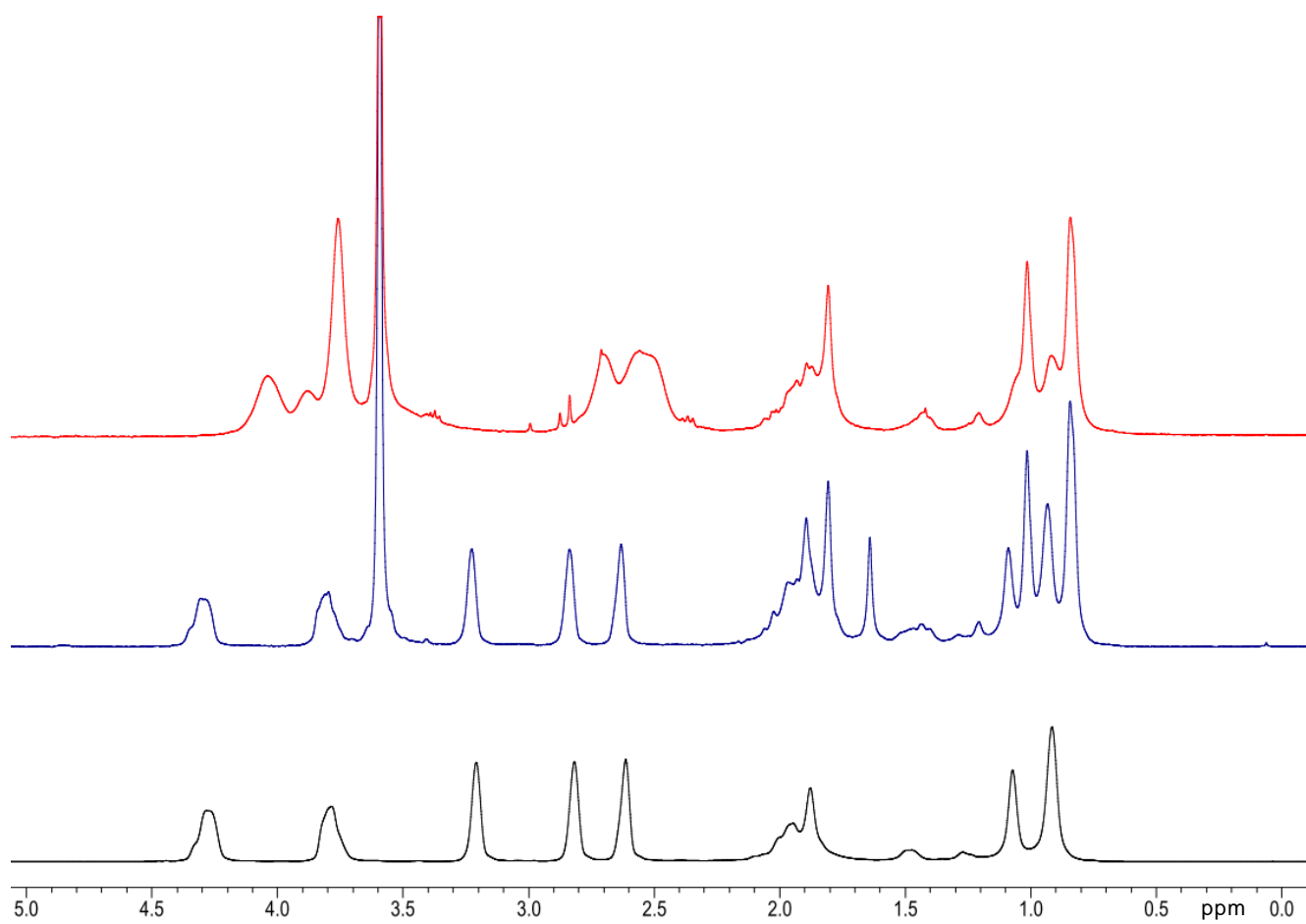
Fig. SI-2 1 H-NMR spectra of PGMA (black line), PGMA- b -PMMA (blue line) and PGMA- b -PHMPMA (red line).
