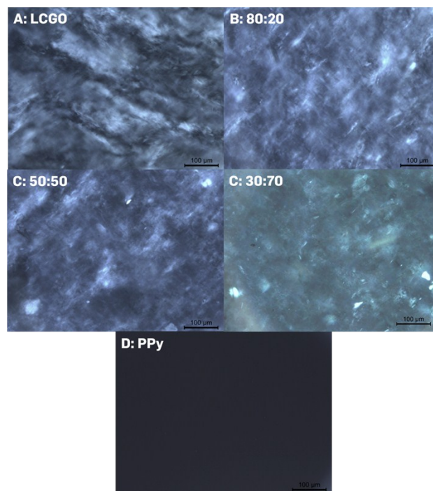
Figure S1: Polarized optical Microscope (POM) images of spinning solution of rGO, PPy and their composites (rGO:PPy).
