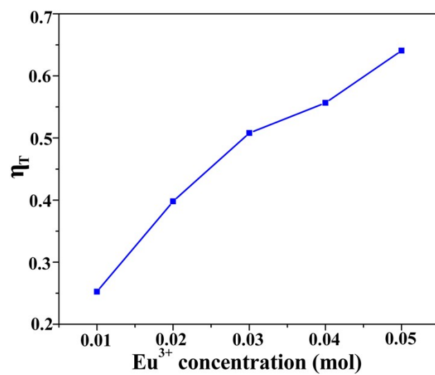
Fig. S1 Energy transfer efficiency from \text{Tb}^{3+} to \text{Eu}^{3+} in V-YOF:0.03 \text{Tb}^{3+} , x\text{Eu}^{3+} ( x = 0\text{--}0.05 ) samples under the excitation of 378 nm.
