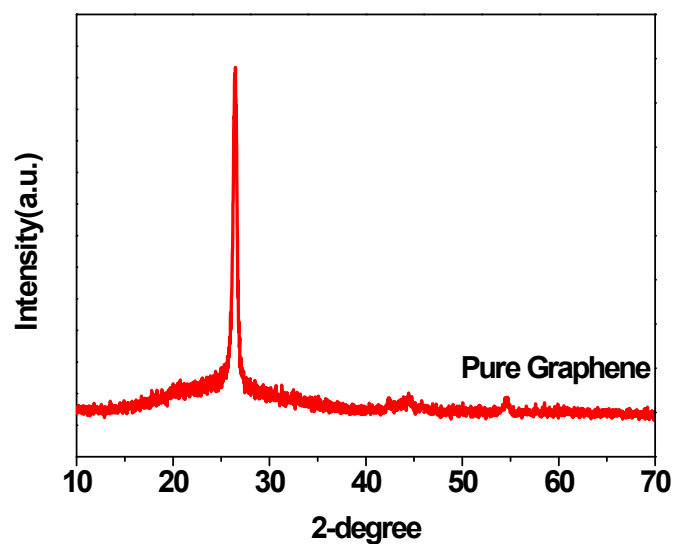
Figure S1. The XRD pattern of the graphene prepared by Hummers method.
