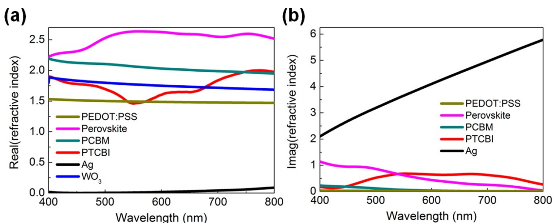
Fig. S1 The real (a) and imaginary (b) part of refractive indices of PEDOT:PSS, perovskite, PCBM, PTCBI, Ag, and WO 3 .
