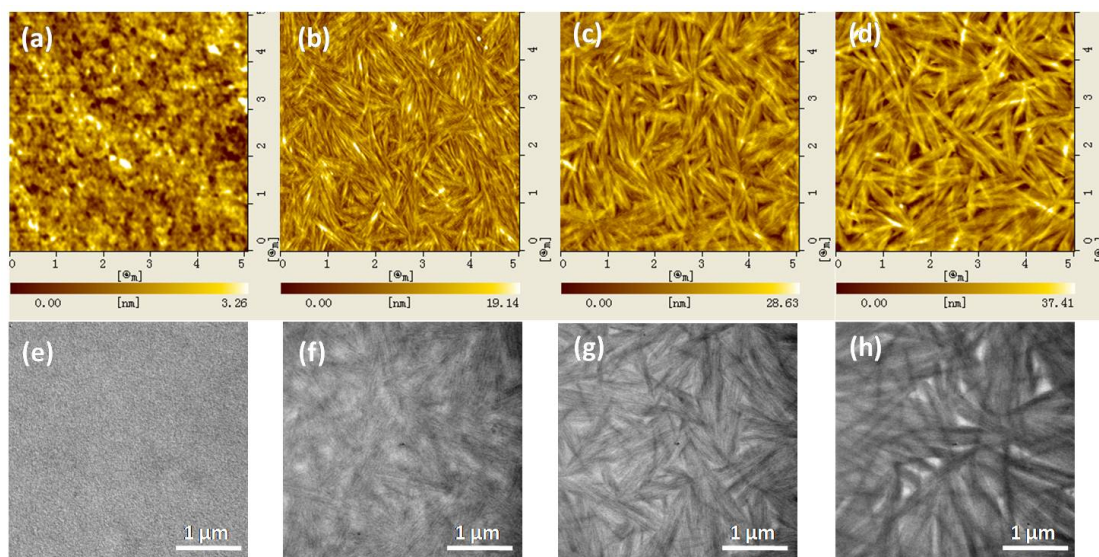
Figure S1. The AFM (a-d) and TEM (e-h) images for the H2:FIrpic(10 wt.%) spin-cast from (a, e) toluene, (b, f) toluene:p-xylene (9:1), (c, g) toluene:p-xylene (5:5), and (d, h) p-xylene solutions.
