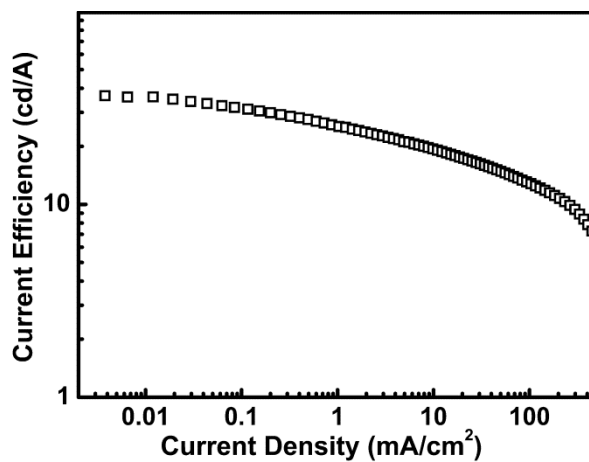
Fig. S3 Current efficiency versus current density of the optimized WOLED.
