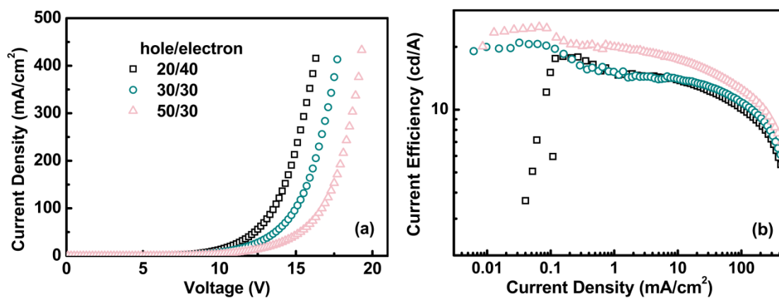
Fig. S2 (a) J-V and (b) current efficiency characteristics of the WOLEDs with different thicknesses of transport layers.
