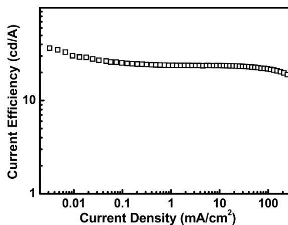
Fig. S1 Current efficiency versus current density of the blue p-i-n homojunction TOLED.
