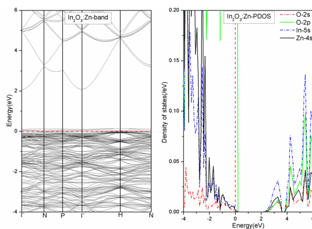
Fig.S1.(a) The bandstructure and (b) PDOS of \text{In}_2\text{O}_3:\text{Zn} , respectively. The red dashed lines in these plots represent Fermi level.
