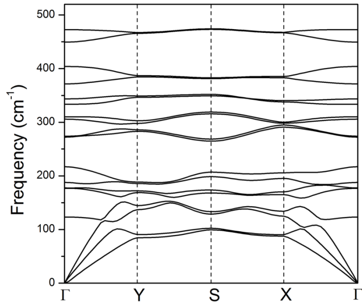
Fig. S1 Phonon spectrum of PdS 2 monolayer.
