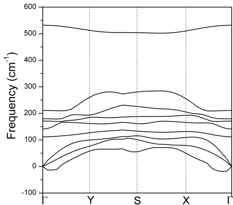
Fig. S3 Phonon spectrum of PdS 2 monolayer with the 2H configuration.
