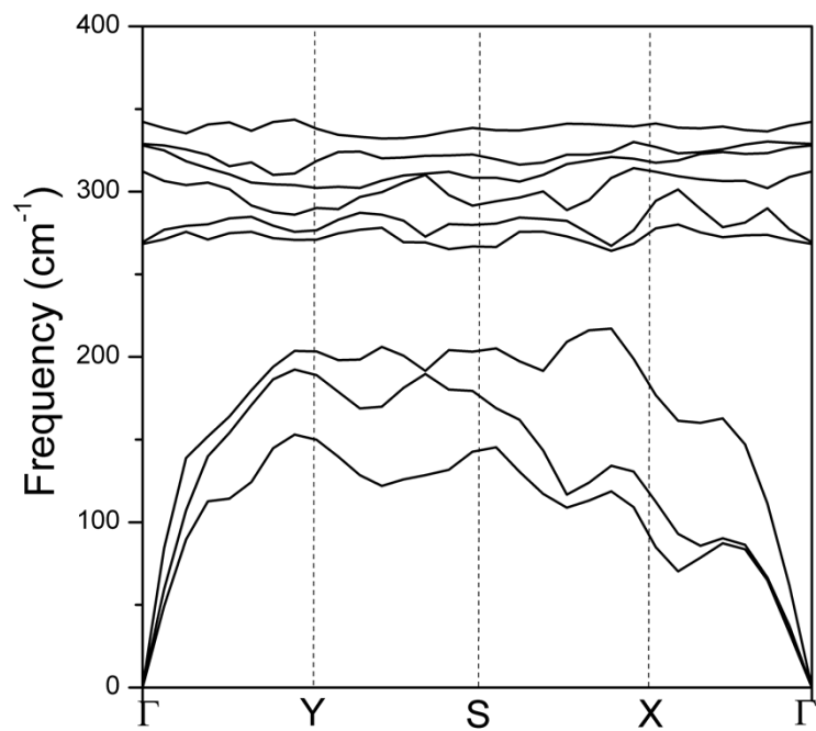
Fig. S2 Phonon spectrum of PdS 2 monolayer with the 1T configuration.
