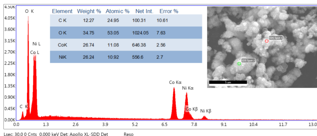
Fig. S1 EDX spectrum of the calcined \text{NiCo}_2\text{O}_4\text{-CoNiO}_2 hybrid at 450 °C.
