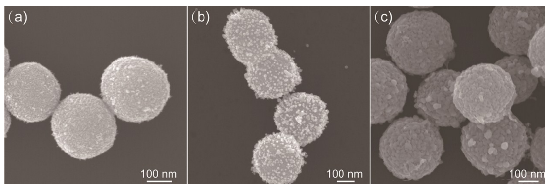
Figure S1. SEM images of \text{Fe}_3\text{O}_4@\text{PEI}@\text{Ag} microspheres synthesized with different amount of \text{AgNO}_3 : (a) 0 mg, (b) 1.5 mg, and (c) 4 mg, respectively.
