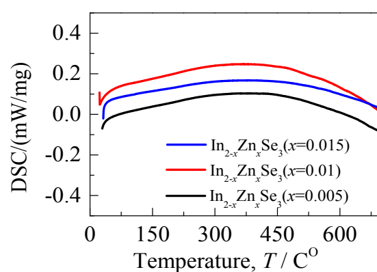
Figure S1 The DTA curves for \text{In}_{2-x}\text{Zn}_x\text{Se}_3 ( x=0.005, 0.01, 0.015 ).
