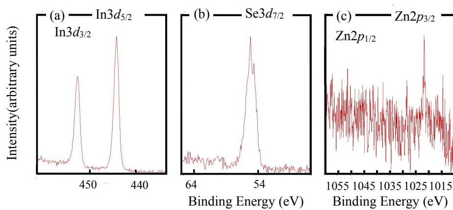
Figure S3 XPS spectra of (a) In 3d, (b) Se 3d, and (c) Zn 2p for \text{In}_{1.99}\text{Zn}_{0.01}\text{Se}_3
