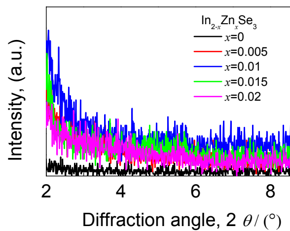
Figure S 4 Small angle X ray diffraction patterns (SAXS) of the \text{In}_{2-x}\text{Zn}_x\text{Se}_3 ( x=0, 0.005, 0.01, 0.015, 0.02 ) powders.
