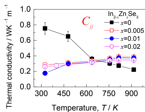
Figure S 5 Total thermal conductivities ( \kappa ) of the \text{In}_2\text{Zn}_x\text{Se}_3 ( x=0, 0.005, 0.01, 0.02 ) along the pressing direction.
