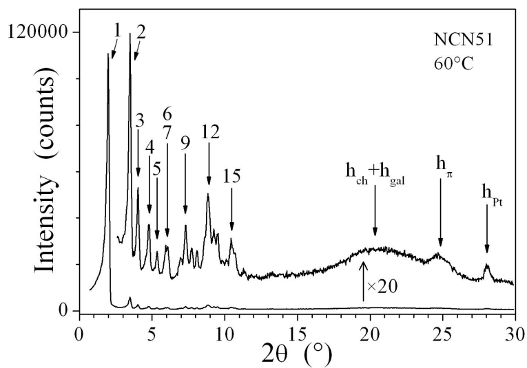
Figure S3: SAXS diffractogram of 7 in the three-dimensional mesophase at 60°C.
