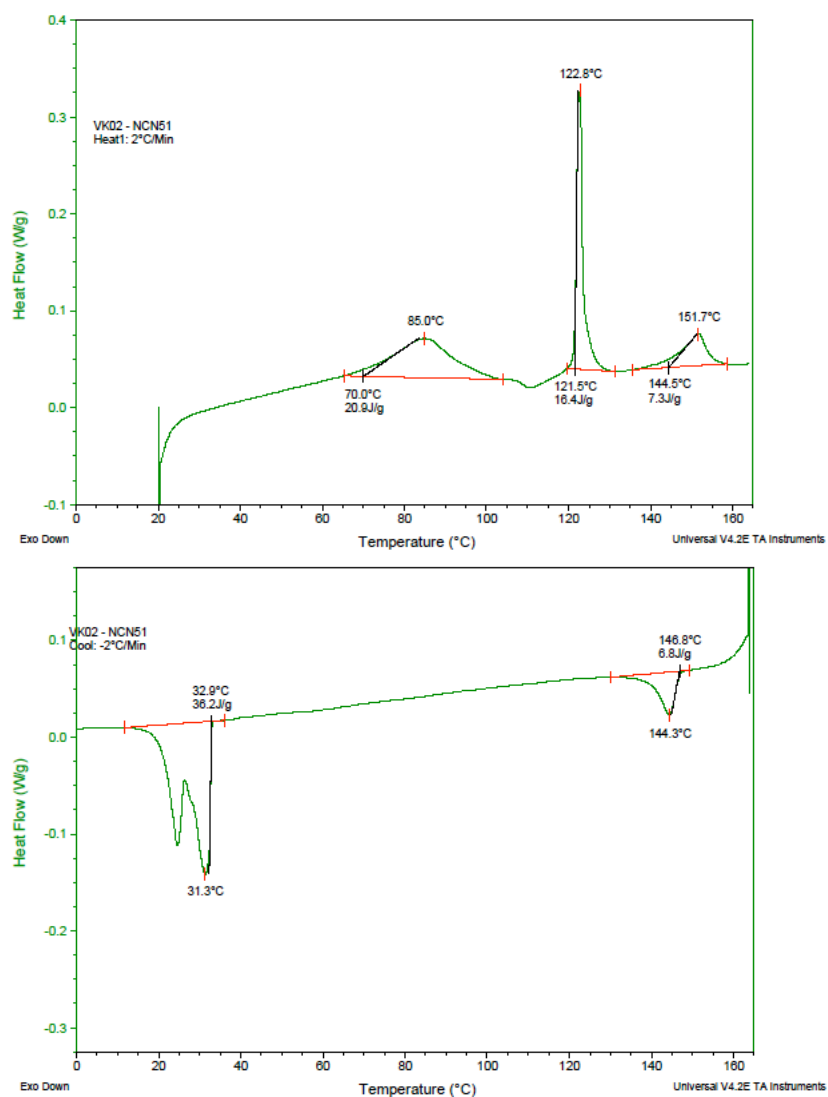
Figure S1: DSC of 7 (1.51 mg, rate 2°C.min -1 ): 1 st heating (top), 1 st cooling (bottom).
