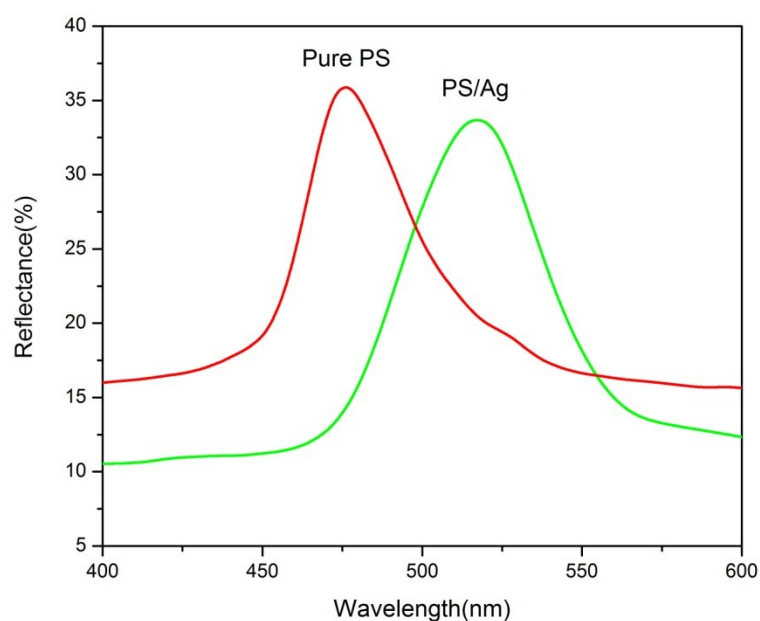
Fig. S1. Reflection spectra of pure PS and PS/Ag-NPs colloidal crystals.
