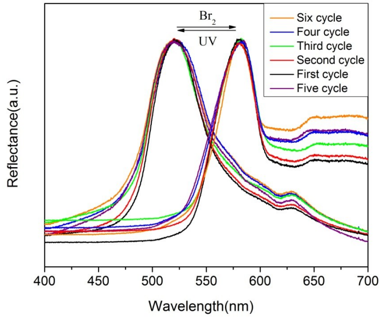
Fig. S2. Reflection spectra of six cycles for bromine gas sensing and regeneration process.
