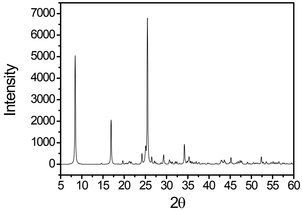
Fig. S1. Simulated X-ray powder diffraction pattern of DBEDOT with strong preferred orientation.
