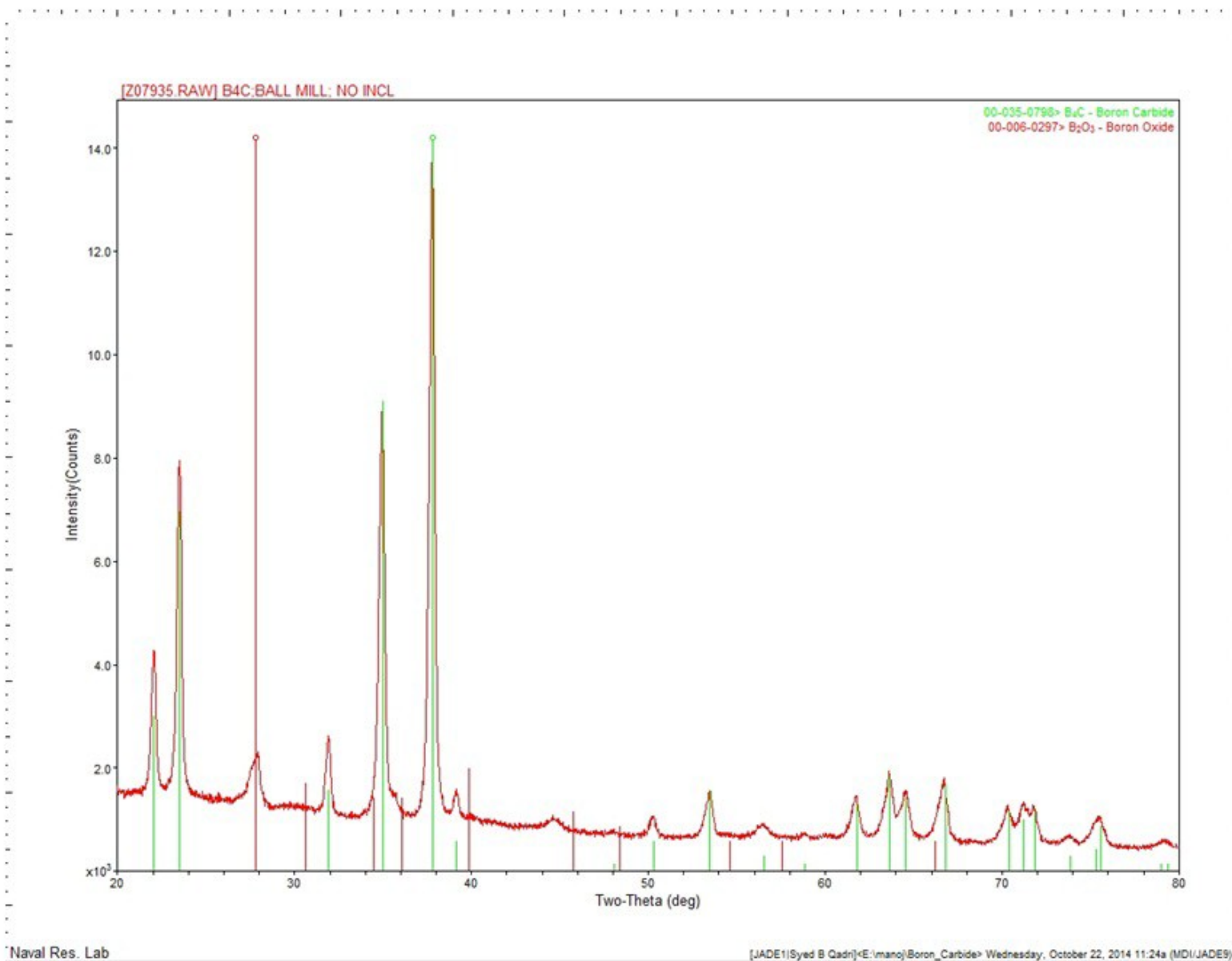
Figure S3: XRD spectrum of the as-received B_4C sample after ball-milling under the same conditions as used during the production of the B_4C:Si sample.
