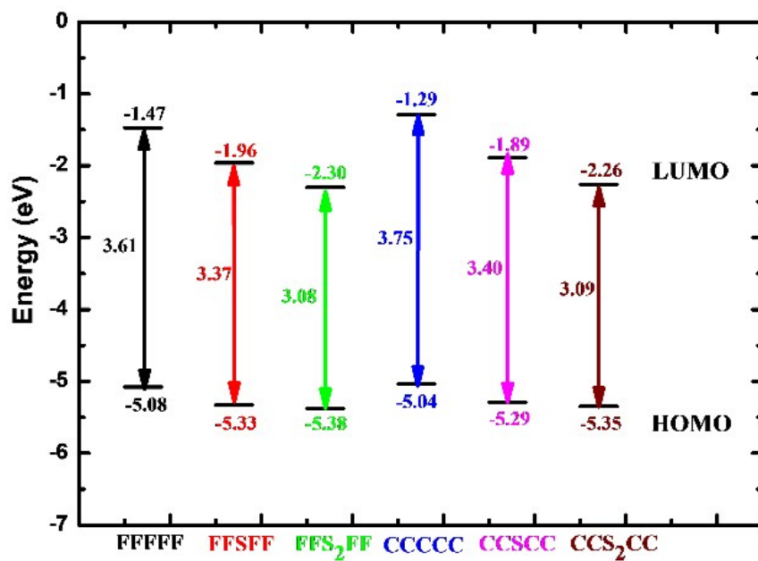
Fig. S6 Energy level diagram for FFFFF, FFSFF, FFS 2 FF, CCCCC, CCSCC and CCS 2 CC.
