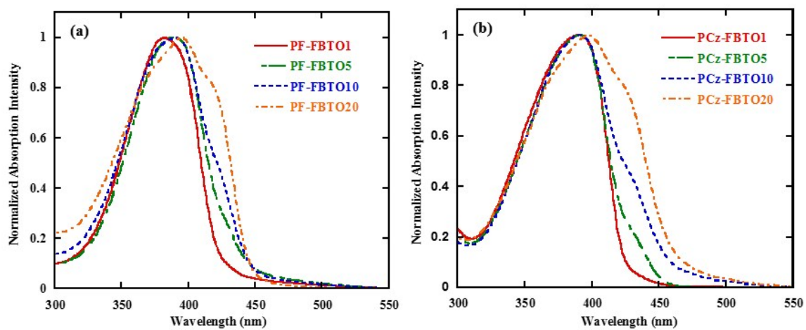
Fig. S4 Absorption spectra of polymers for PF-FBTOs (a) and PCz-FBTOs (b) in film.
