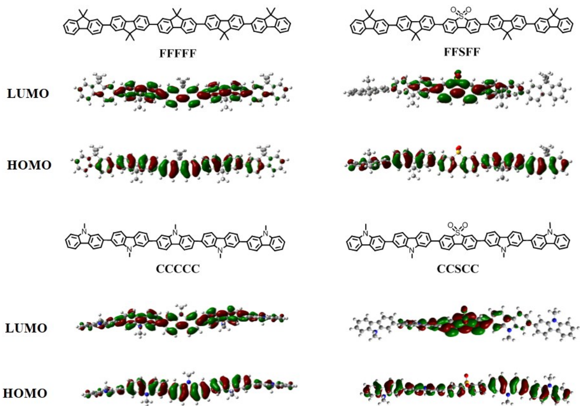
Fig. S5 Structure and spatial distribution of HOMO and LUMO in model molecules.
