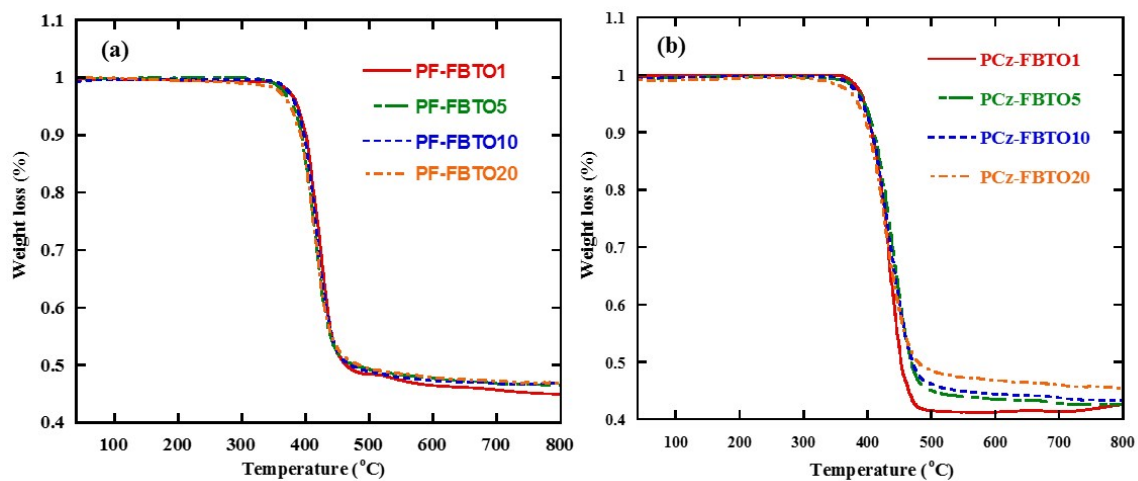
Fig. S2 TGA curves of copolymers PF-FBTOs and PCz-FBTOs.
