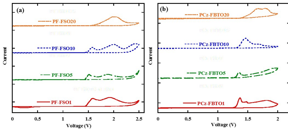
Fig. S3 Cyclic voltammetry curves of PF-FBTOs (a) and PCz-FBTOs (b)
