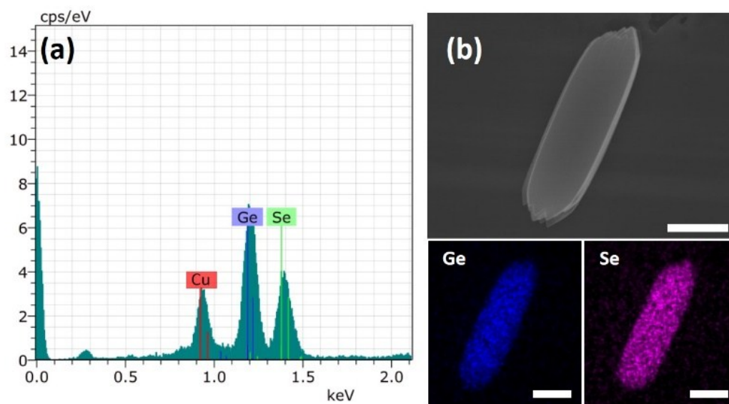
Fig. S3 EDS spectrum and elemental mapping images of GeSe nanosheets.
