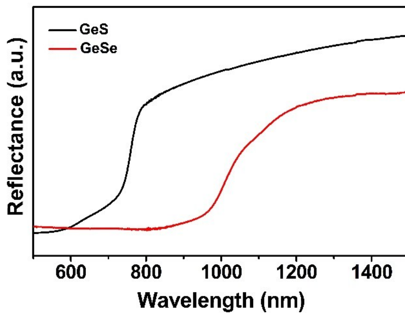
Fig. S4 Diffuse reflectance spectra of GeS and GeSe nanosheets.
