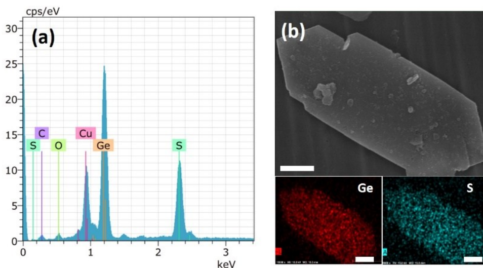
Fig. S2 EDS spectrum and elemental mapping images of GeS nanosheets.
