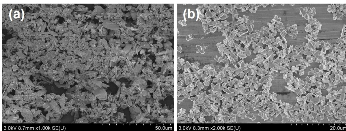
Fig. S1 SEM images of (a) GeS and (b) GeSe nanosheets.
