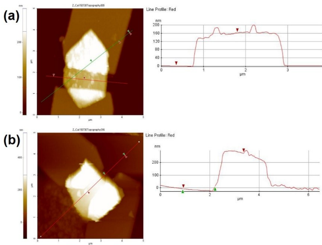
Fig. S5 AFM images of (a) GeS and (b) GeSe photodetectors.
