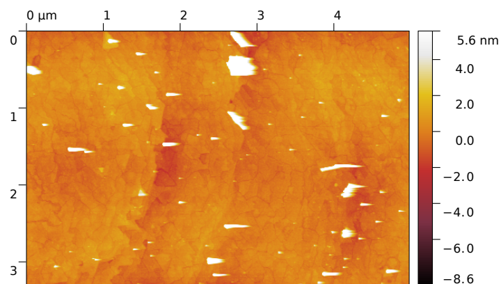
Figure S1: AFM image of a 4.7 nm thick FeO film grown on Ru(0001).
