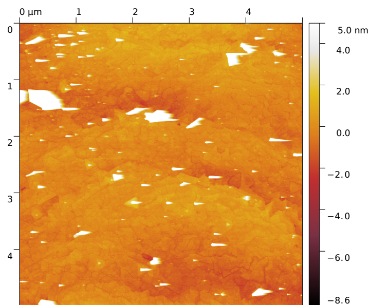
Figure S2: AFM image of a 4.7 nm thick FeO film grown on Ru(0001).
