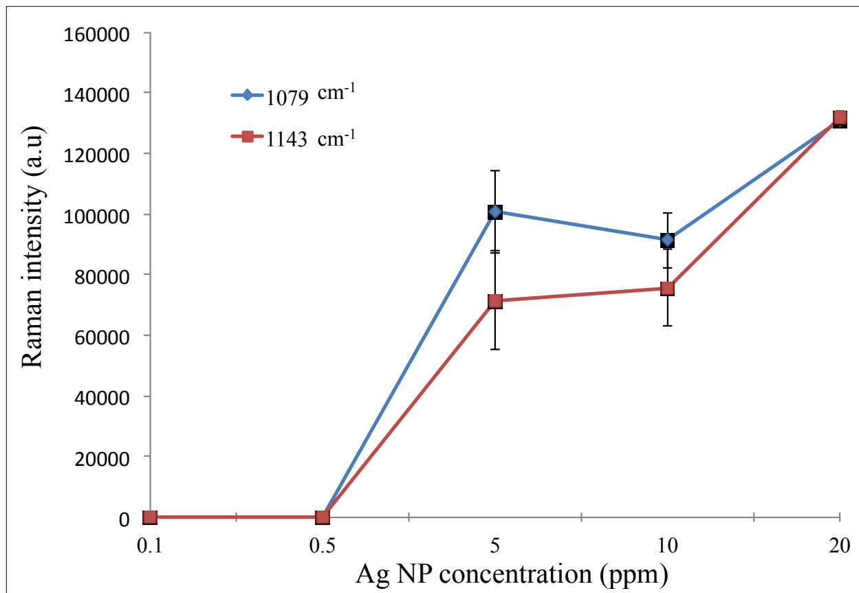
Figure S1. SERS intensity of Ag NPs (20 nm) conjugated with PATP at 1079 and 1143 \text{cm}^{-1} .
