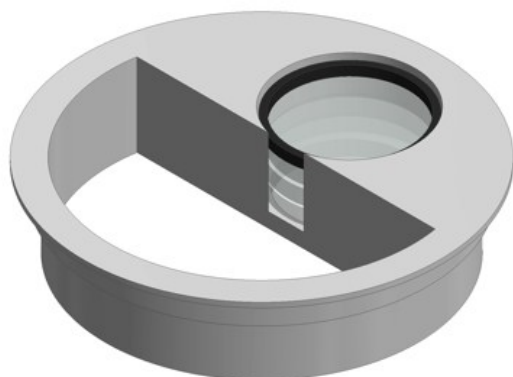
Figure S1 : 3D modelisation of the filter adapter used on the neurosurgical microscope. The piece was 3D printed using white ABS plastic and the three filters were placed in the circular hole and held in place using a retaining ring
