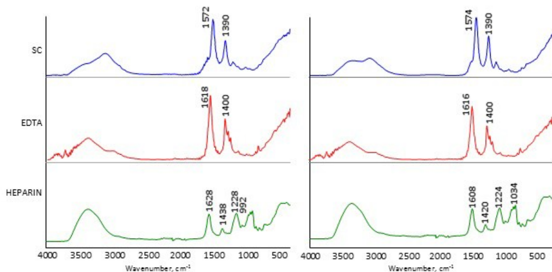
Supplementary Figure 1 Raw spectra of anticoagulants from extracted from blood vials (left) and analytical grade compound (right).
