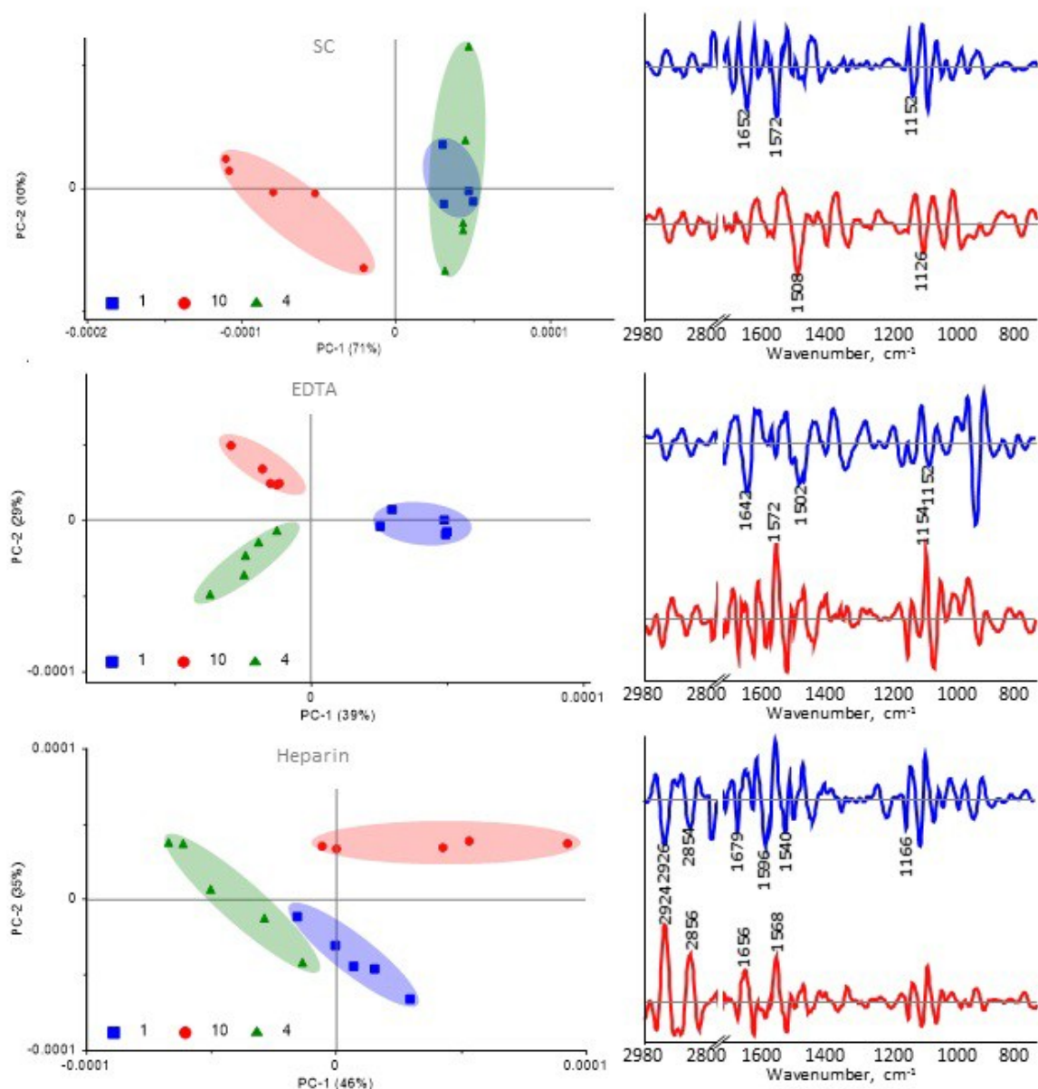
Supplementary Figure 3 Scores for wet plasma spectra collected in vials containing SC (top), EDTA (middle) or Heparin (bottom). To the left of the scores are the corresponding PC1 (blue) and PC2 (red) loadings. In all cases, there is little difference between 1 h and 4 h, however at 10 h there is a significant difference.
