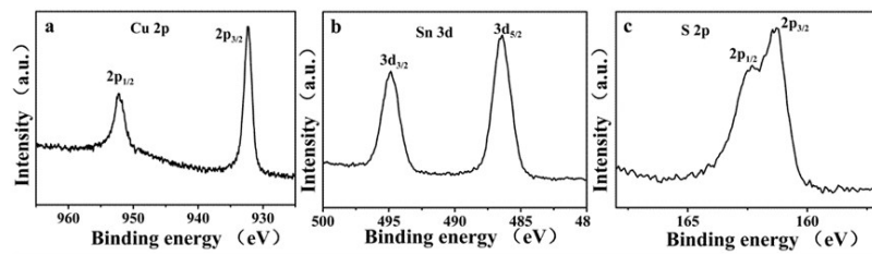
Figure S3. XPS spectra of \text{Cu}_2\text{SnS}_3 nanocrystals.
