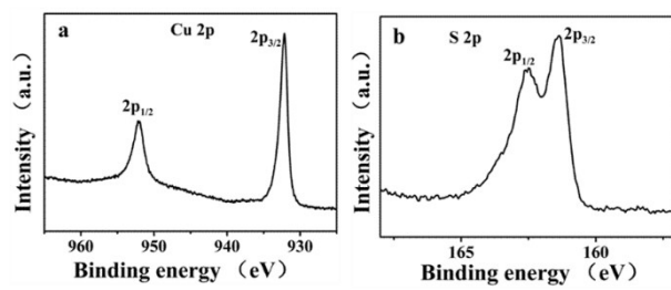
Figure S2. XPS spectra of Cu 2 S nanocrystals.
