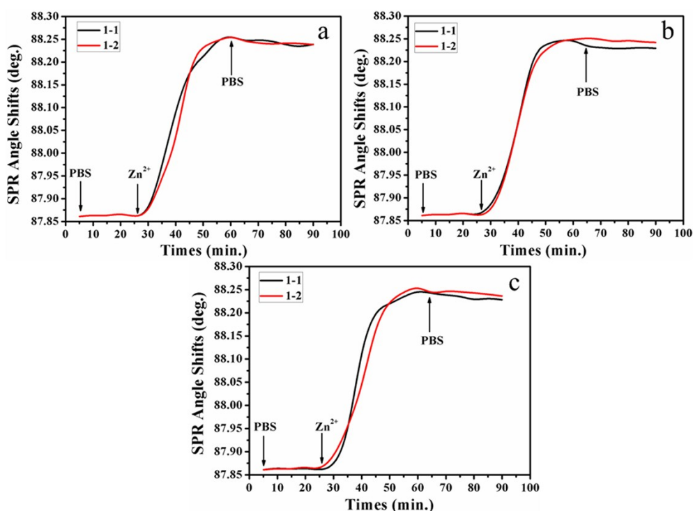
Figure S1 The original SPR data for real samples detection. (a) Urine, (b) Tap water and (c) Pond water: black line (0.1 μM) and red line (1 μM).
