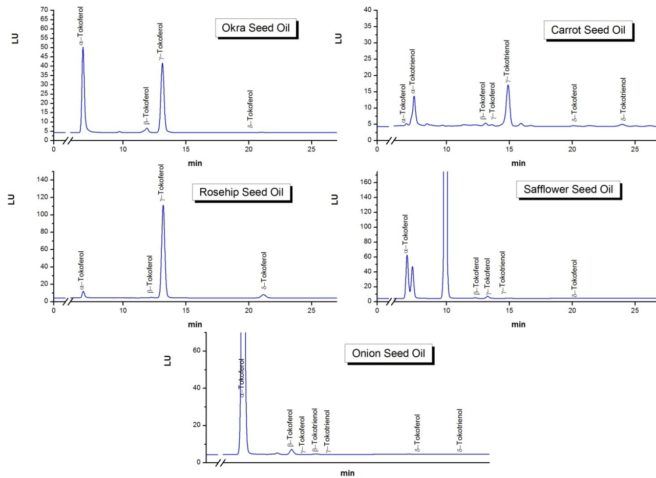
Fig. S2. The tocol chromatograms for onion, okra, rosehip, safflower and carrot seed oils
