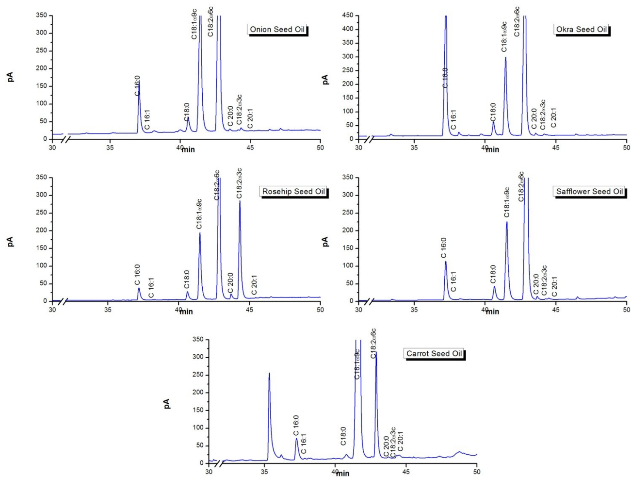
Fig. S1. The fatty acid (FA) composition chromatograms for onion, okra, rosehip, safflower and carrot seed oils
