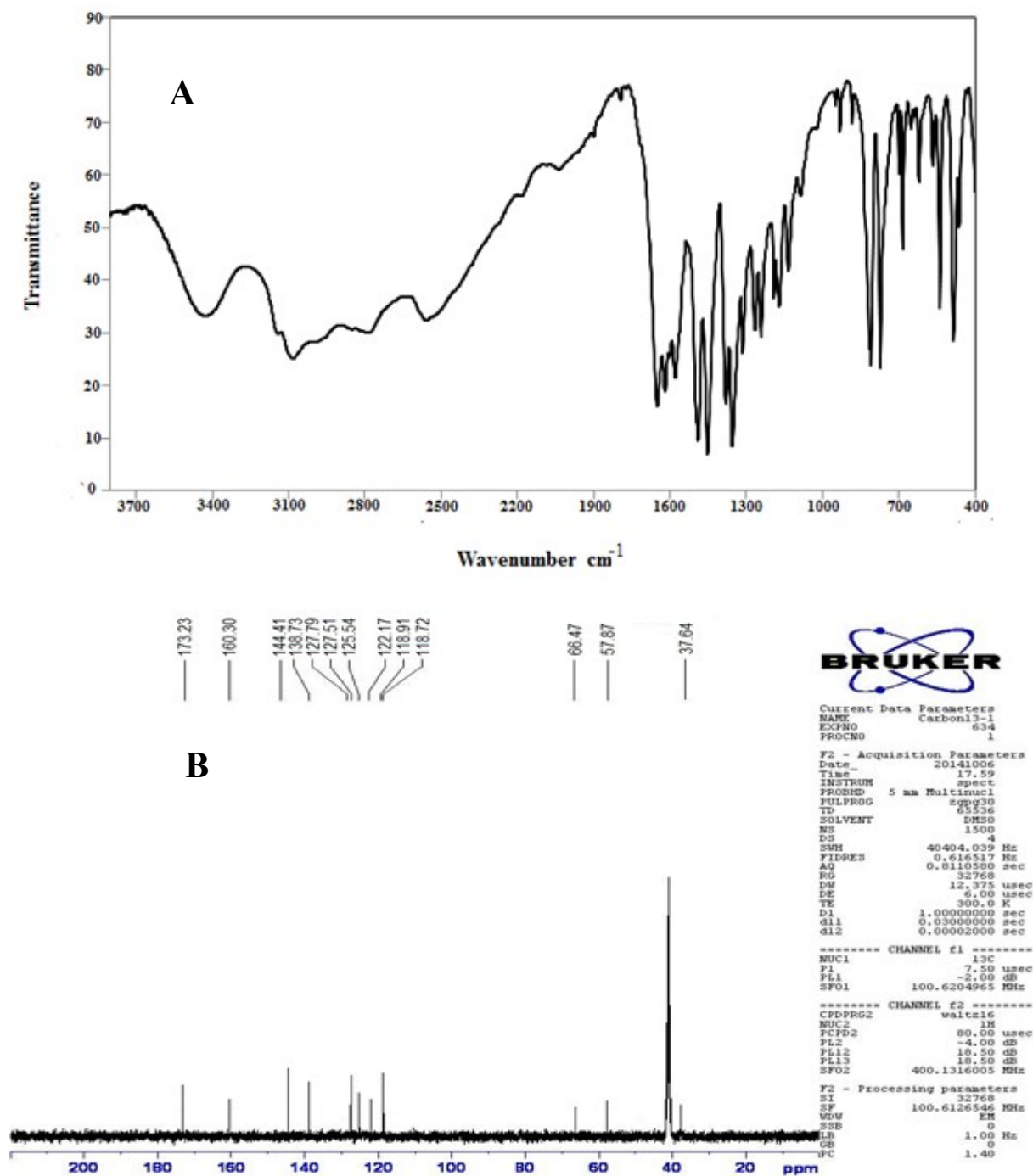
(A) FTIR and (B) ^{13}\text{C} NMR spectra of [5-ASA- \text{C}_1\text{C}_2\text{Im} ][Br]
