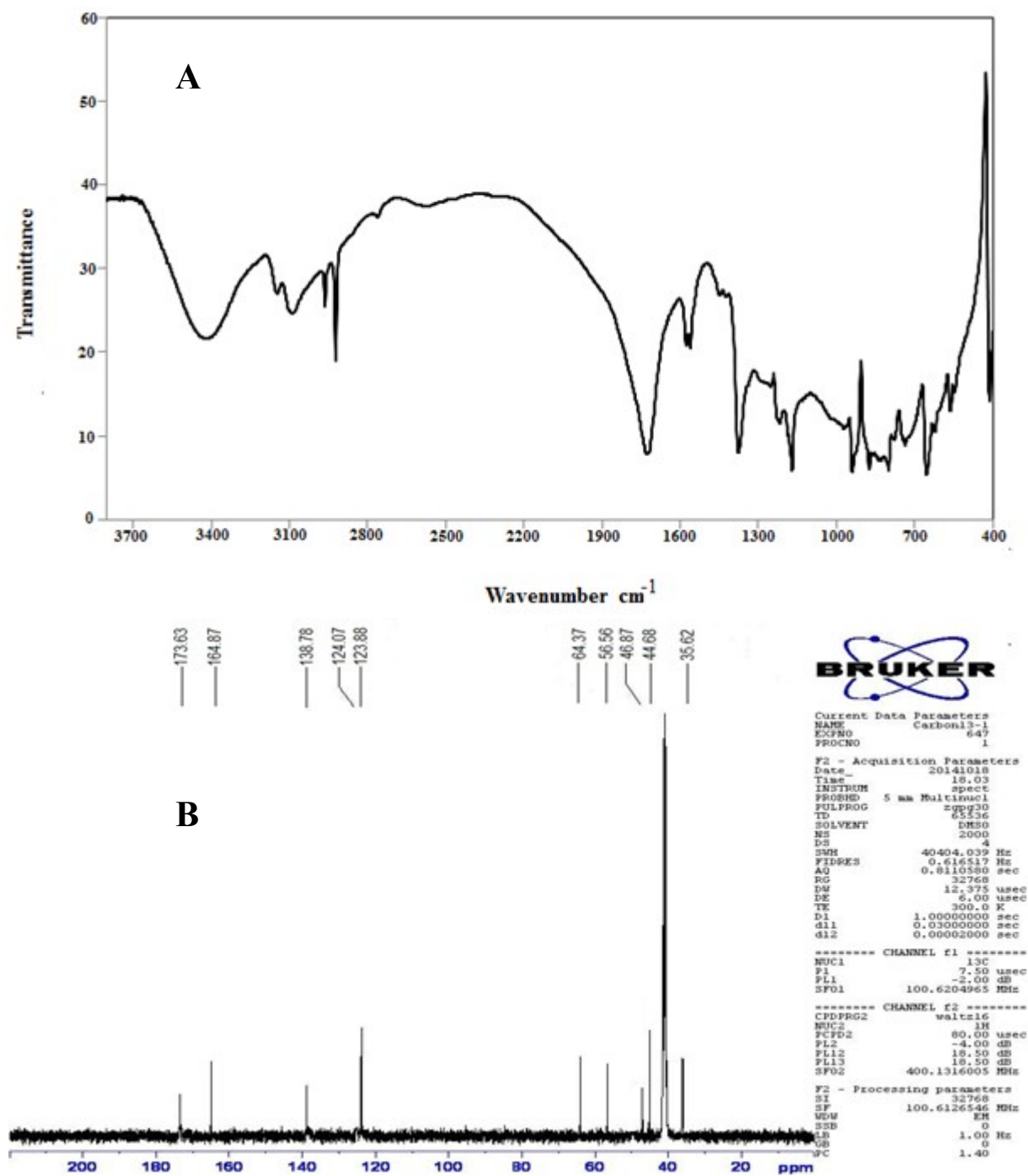
(A) FTIR and (B) 13 CNMR spectra of [TH-C 1 C 2 Im][Br]
