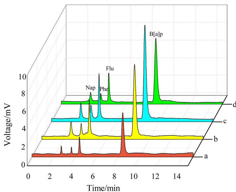
Fig. S2 Typical chromatograms of different fibers with AuNPs electrodeposited within 5 min (a), 10 min (b), 15 min (c) and 20 min (d). Conditions: Temperature, 45 °C; Stirring, 350 r/min; Extraction, 30 min; Desorption, 5 min; Nap, Phe, Flu and B[a]p, 50 µg/L.
