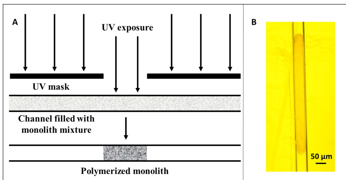
Figure S1. Monolith fabrication. (A) Schematic showing monolith fabrication via UV polymerization. (B) Photograph of a C8 monolith polymerized in a channel that has been filled with a 1:1 IPA:water mixture.
