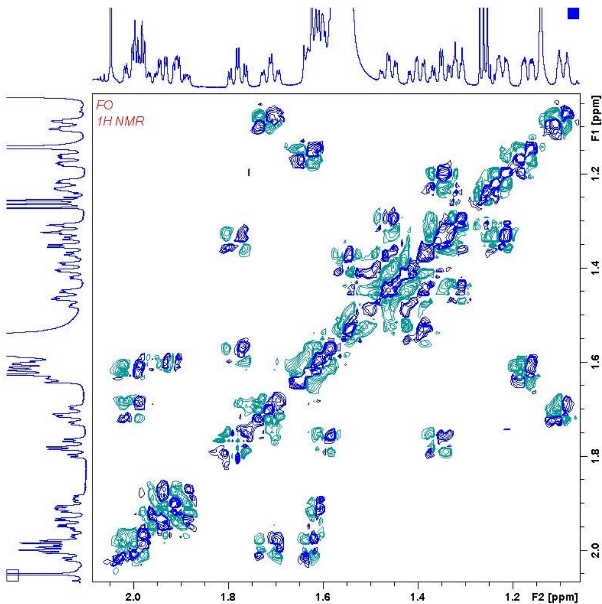
Fig S1. DQF-COSY spectrum of maslinic acid in \text{CDCl}_3 solution
