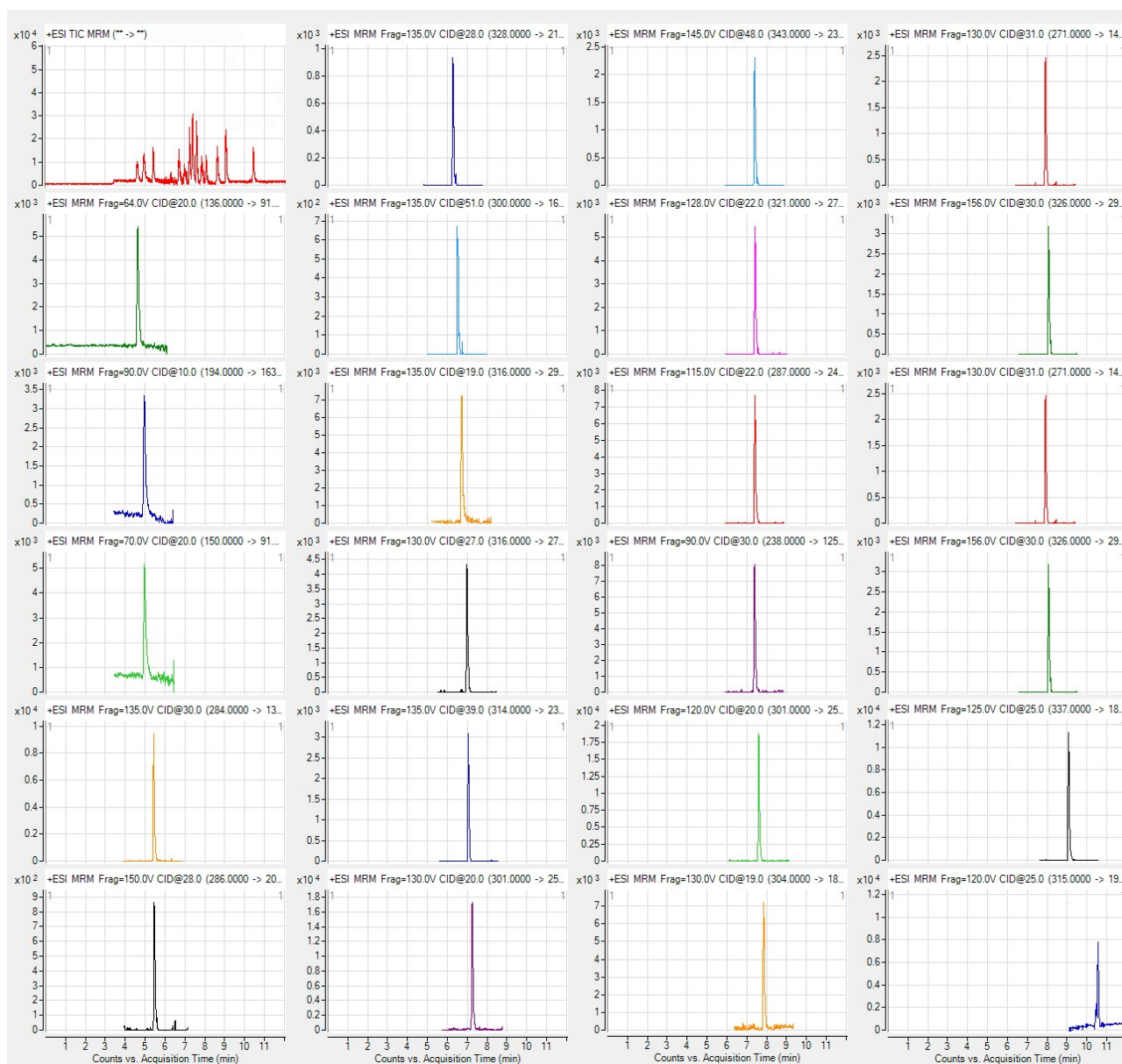
TIC for all 23 analytes and individual MRMs for each analyte for 3 ng/mL standard on 2.6 \mu\text{m} HPH column
