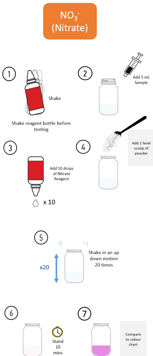
Figure A: Pictograph instructions for carrying out the developed nitrate method
