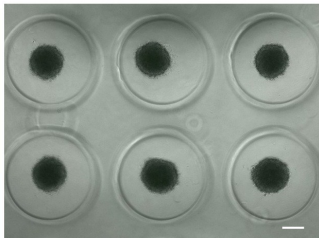
Sox2-GFP
