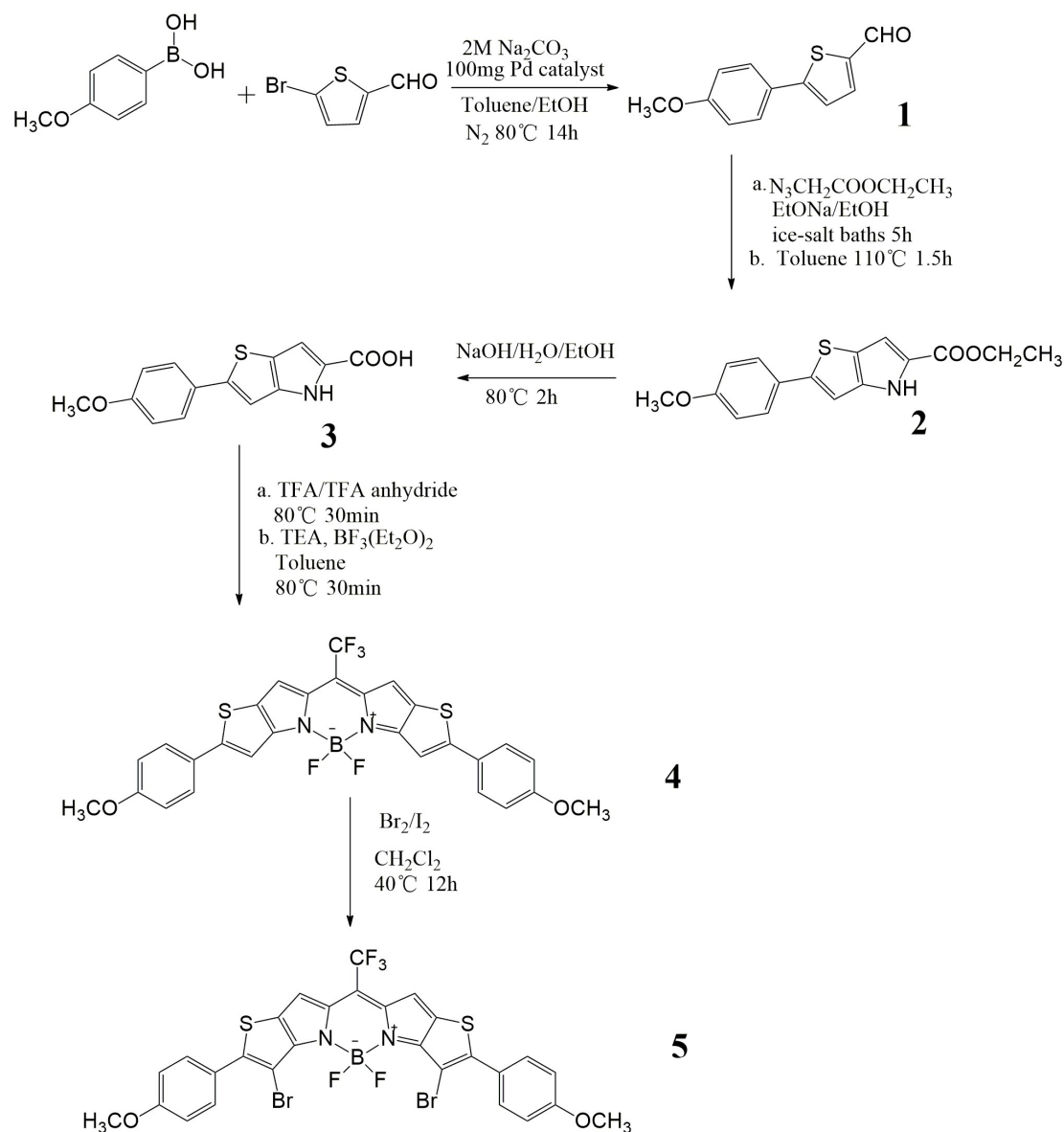
Scheme S1. Synthesis of the BODIPY
