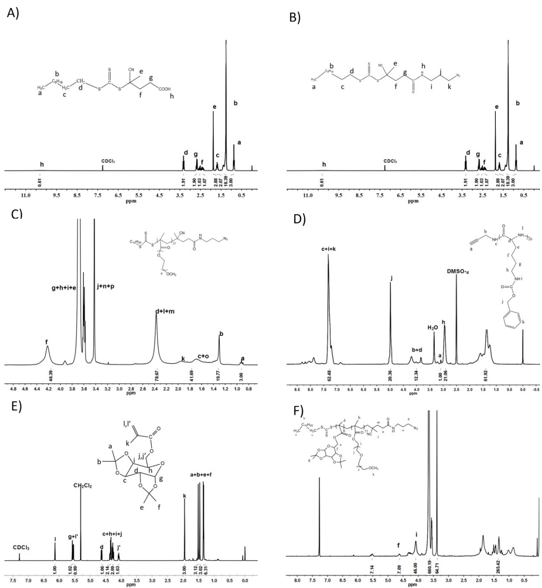
Figure S1. ^1\text{H} -NMR of polymer synthesis: (A)RAFT-1, (B)RAFT, (C)POEGMA, (D)PLys, (E) MALpGP and (F)PMAIpGP-POEGMA.
