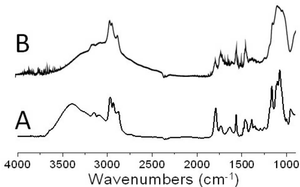
Figure S1. ATR-FTIR spectra of SIM A) before irradiation and B) after 1200s of irradiation
