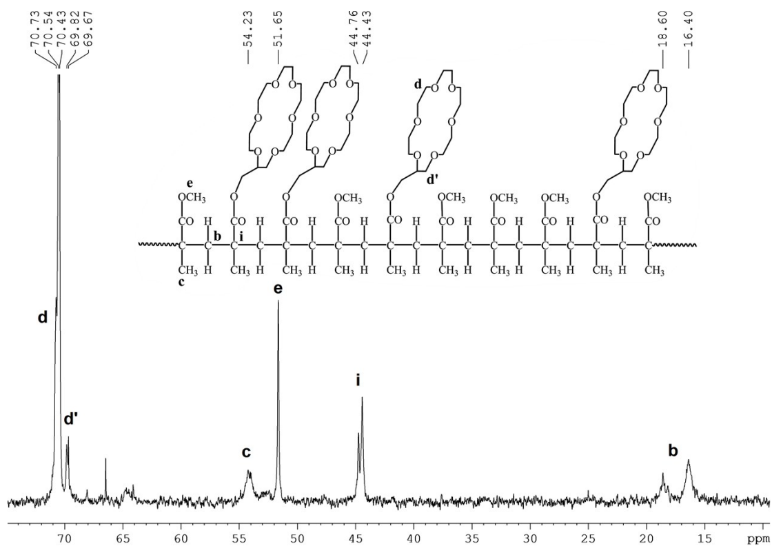
Figure S2. ^{13}\text{C} -NMR spectrum of PMMA-ran-PACM-18CE, BC copolymer ( \text{CDCl}_3 , 400 MHz, 298K)
