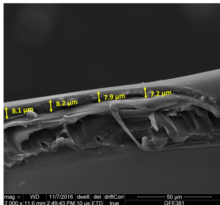
Figure S1: SEM image of the dried indicator film, with a thickness of ca. 8 microns
