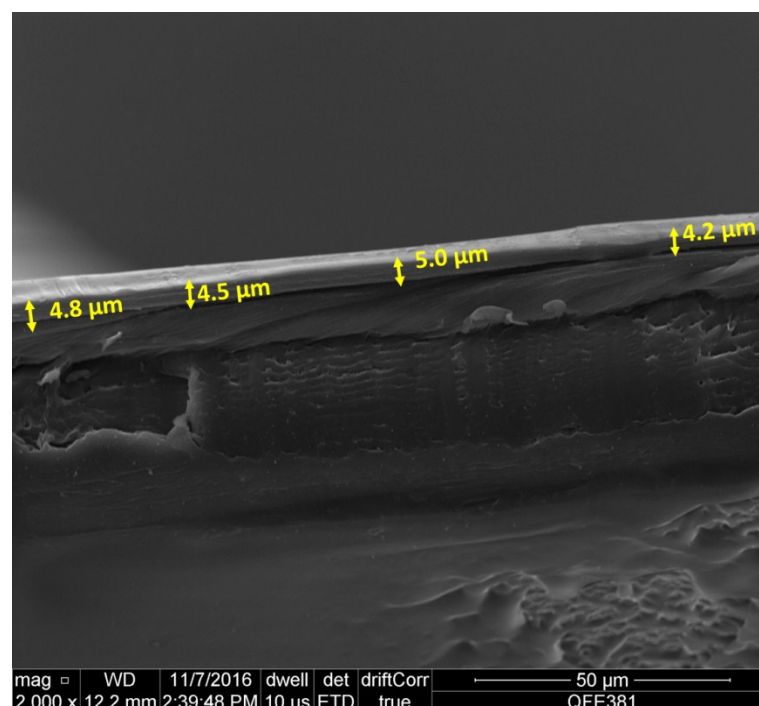
Figure S2: SEM image of the dried ammonia-generating adhesive film, with a thickness of ca. 5 microns
