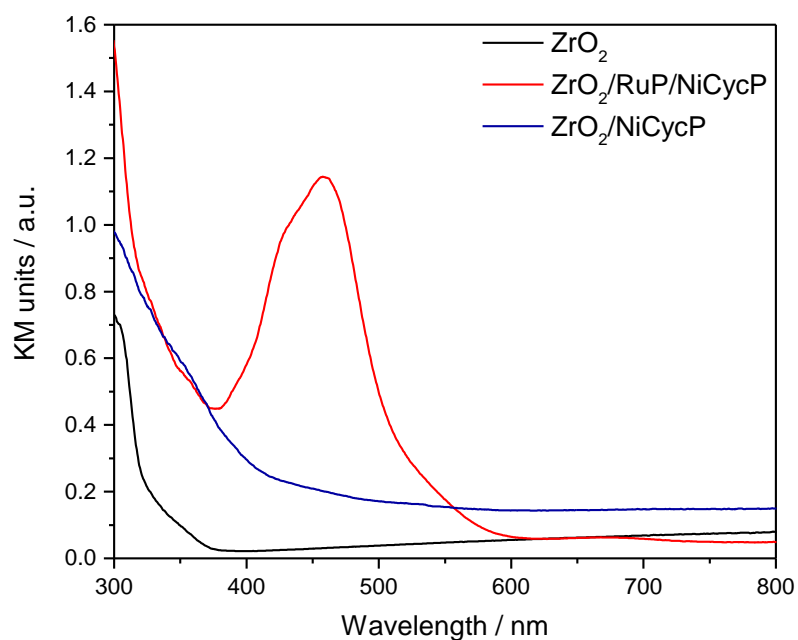
Figure S4 - DR UV/Vis spectra of \text{ZrO}_2/\text{RuP}/\text{NiCycP} powders used in the photocatalysis studies, transformed using the Kubelka-Munk function
