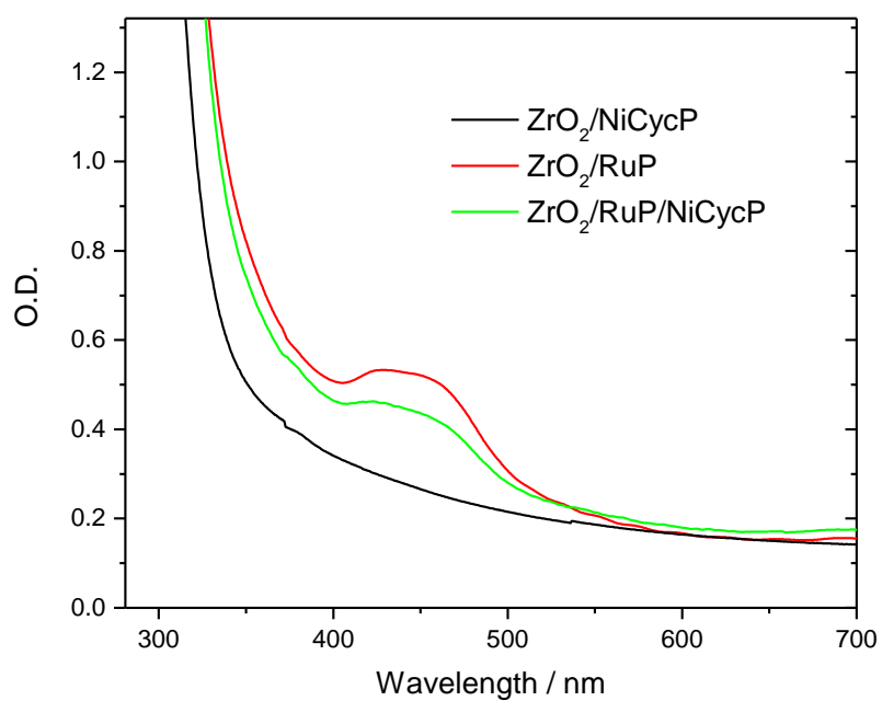
Figure S3 - UV/Vis spectra of \text{ZrO}_2/\text{NiCycP} , \text{ZrO}_2/\text{RuP} and \text{ZrO}_2/\text{RuP}/\text{NiCycP} films.
