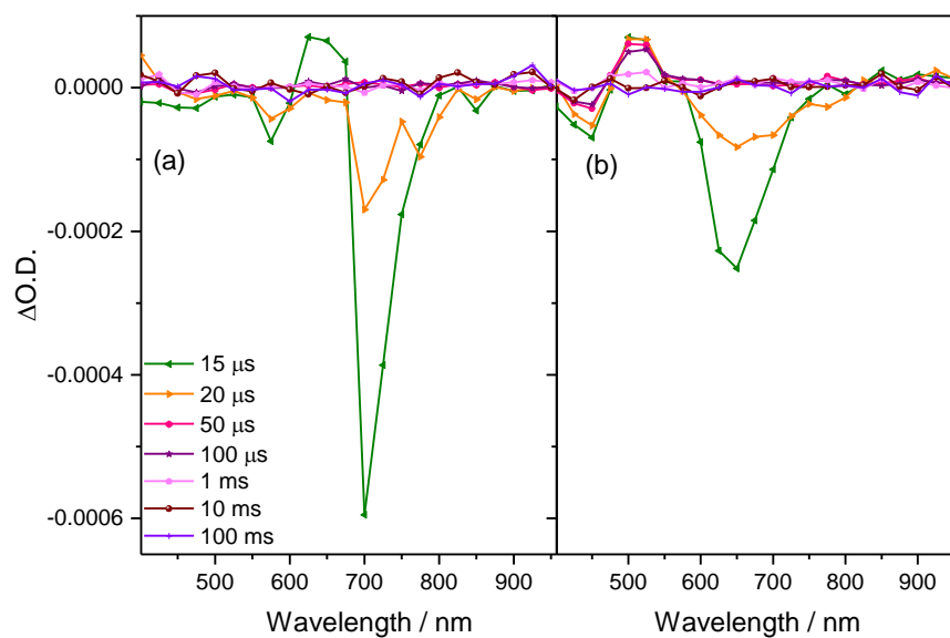
Figure S15 - TA spectra of \text{ZrO}_2/\text{Ru P} in \text{H}_2\text{O} (a) and (b) 0.1 \text{ M} ascorbate (pH 4) following 355 \text{ nm} (6 ns) excitation at the time delays indicated.
