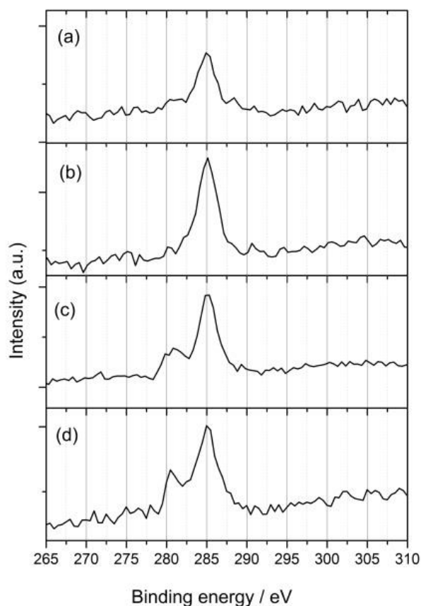
Figure S9 - Low resolution XPS spectra of Ru 3d region for (a) \text{ZrO}_2 , (b) \text{ZrO}_2/\text{NiCycP} , (c) \text{ZrO}_2/\text{NiCycP}/\text{RuP} , (d) and \text{ZrO}_2/\text{NiCycP}/\text{RuP} post catalysis showing the presence of the \text{Ru}^{2+} in the post catalysis (48 hr) sample.
