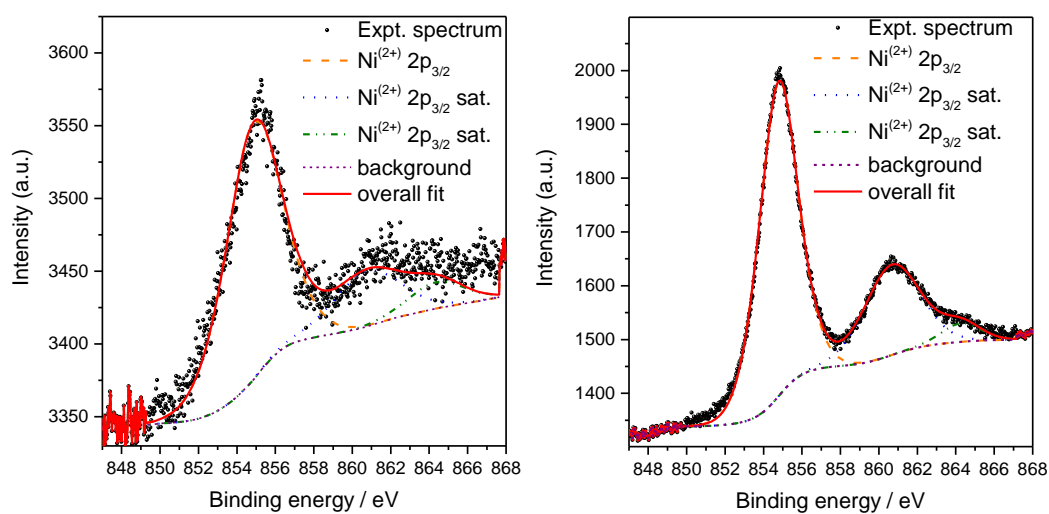
Figure S10 - Experimental and simulated XPS spectra of Ni 2p levels for \text{ZrO}_2/\text{NiCycP} (left) and \text{NiCycP} (right)
