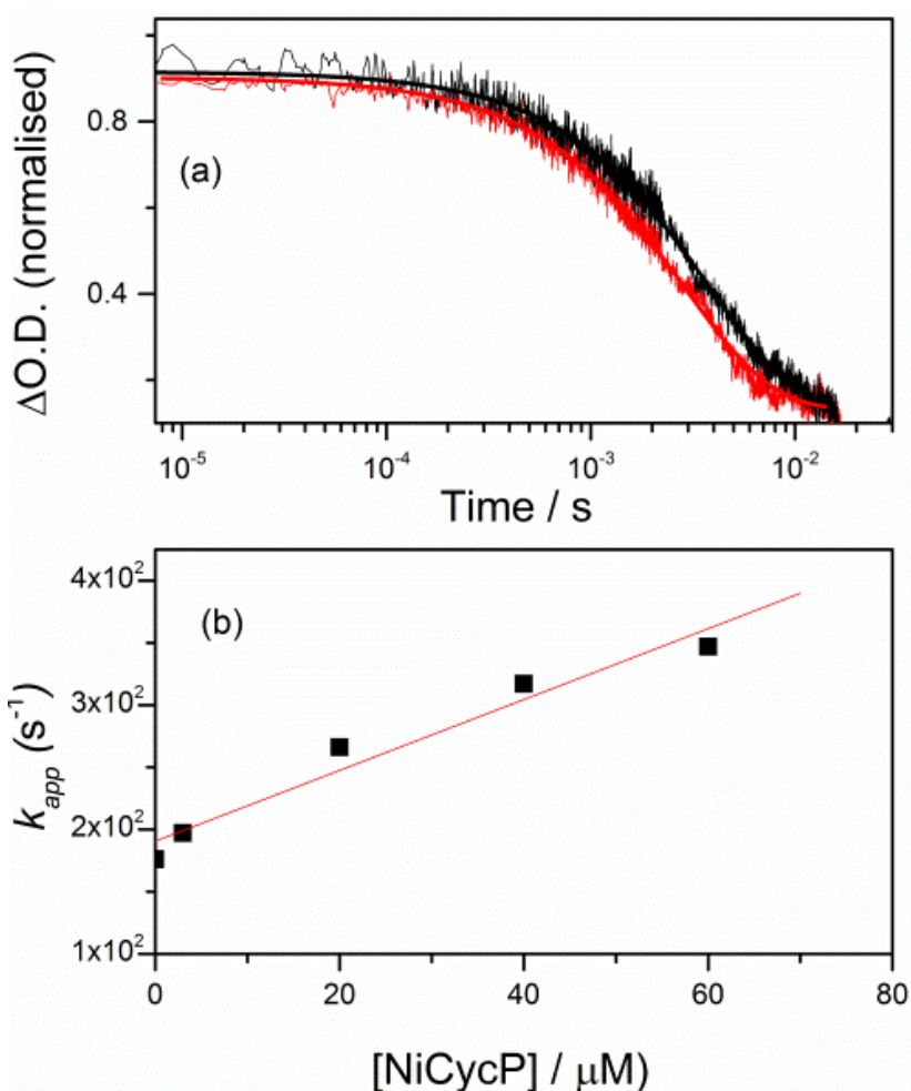
Figure S16 - (a) Kinetic traces recorded at 510 nm of RuP * in solution formed following 355 nm excitation of RuP (9 \mu M ) in a argon purged 0.1 M ascorbate in the absence (black line) and presence of NiCycP (60 \mu M , red line). (b) NiCycP concentration dependence for the apparent rate constant of RuP * loss ( k_{app} ) in solution.
