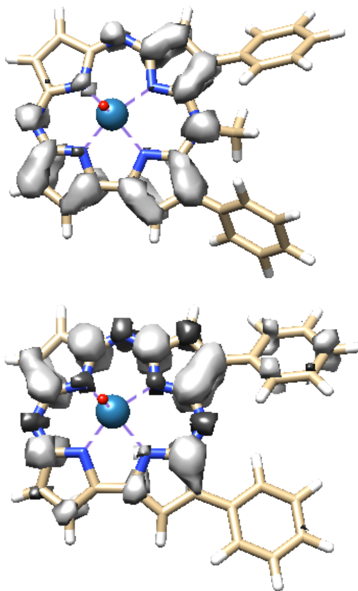
Figure S16. Spin density plot for ^2[\text{Re}^{\text{V}}(\text{O})(\text{CzH}_6\text{P}_2)(\text{CH}_3)]^\bullet (top) and ^2[\text{Re}^{\text{V}}(\text{O})(\text{CzH}_6\text{P}_2)]^{\bullet+} (bottom) at the PBE0/SDD/6-31G** level of theory. Positive (grey) and negative (black) spin densities are shown at the isodensity level of 0.002 electron/bohr.
