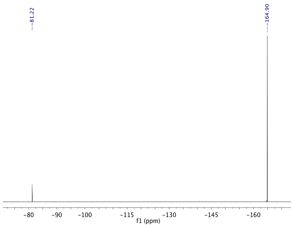
Figure S2. ^{19}\text{F} NMR spectrum of [\text{Re}^{\text{V}}(\text{O})(N\text{-MeTBP}_8\text{Cz})]^+[\text{OTf}]^- ( 1 ) in \text{CD}_2\text{Cl}_2 . Chemical shifts were calibrated versus the standard \text{C}_6\text{F}_6 at -164.9 ppm.
