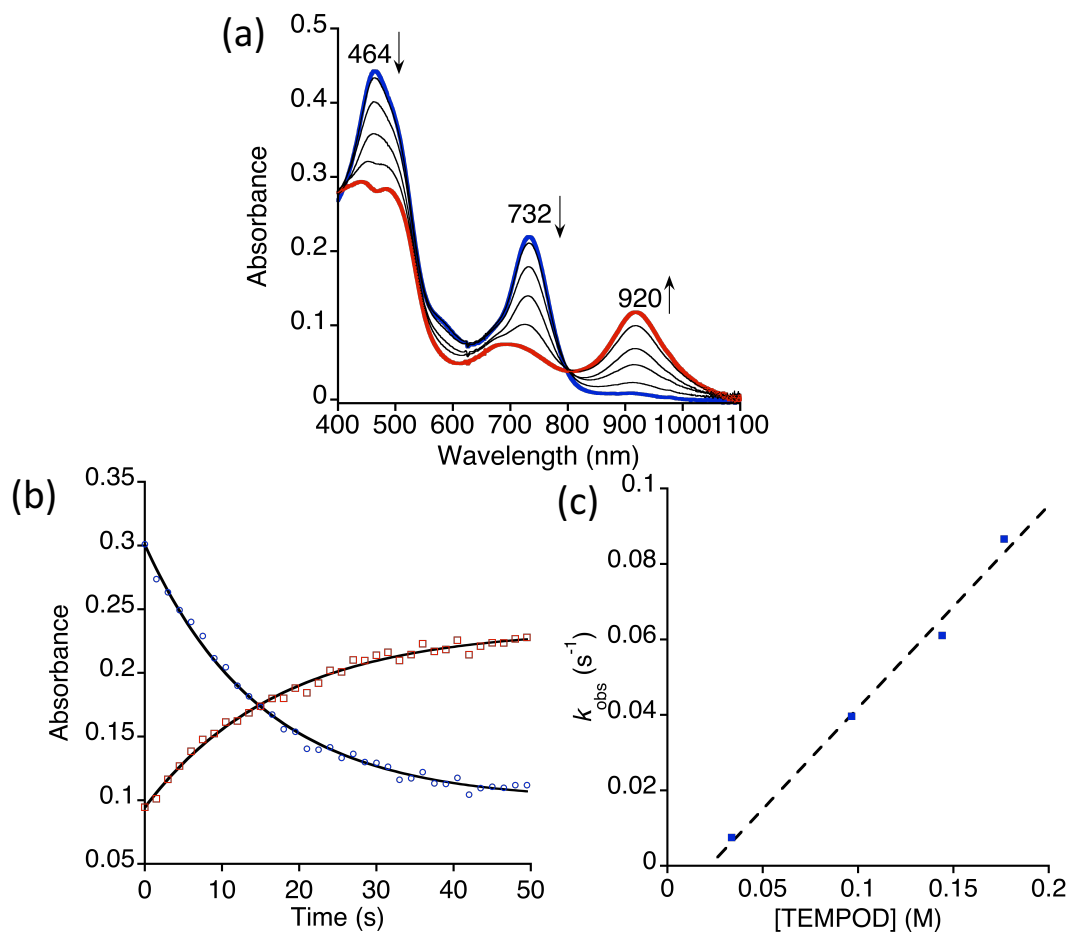
Figure S14. a) Time-resolved UV-vis spectral changes observed for the reaction of [\text{Re}^{\text{V}}(\text{O})(\text{N-MeTBP}_8\text{Cz})]^+[\text{OTf}]^- ( 1 ) (13 \mu\text{M} ) with TEMPOD (0.14 M) in \text{CH}_2\text{Cl}_2 at 25 ^\circ\text{C} . b) Plot of the change in absorbance vs time for the growth of [\text{Re}^{\text{V}}(\text{O})(\text{N-MeTBP}_8\text{Cz})]^\bullet (red squares) and decay of [\text{Re}^{\text{V}}(\text{O})(\text{N-MeTBP}_8\text{Cz})]^+[\text{OTf}]^- ( 1 ) (blue circles) with the best fit lines (black). c) Plot of pseudo-first-order rate constants ( k_{\text{obs}} ) vs [\text{TEMPOD}] ( R^2 = 0.99 ). Slope: k_2 = 0.54(4) \text{ M}^{-1} \text{ s}^{-1} .
