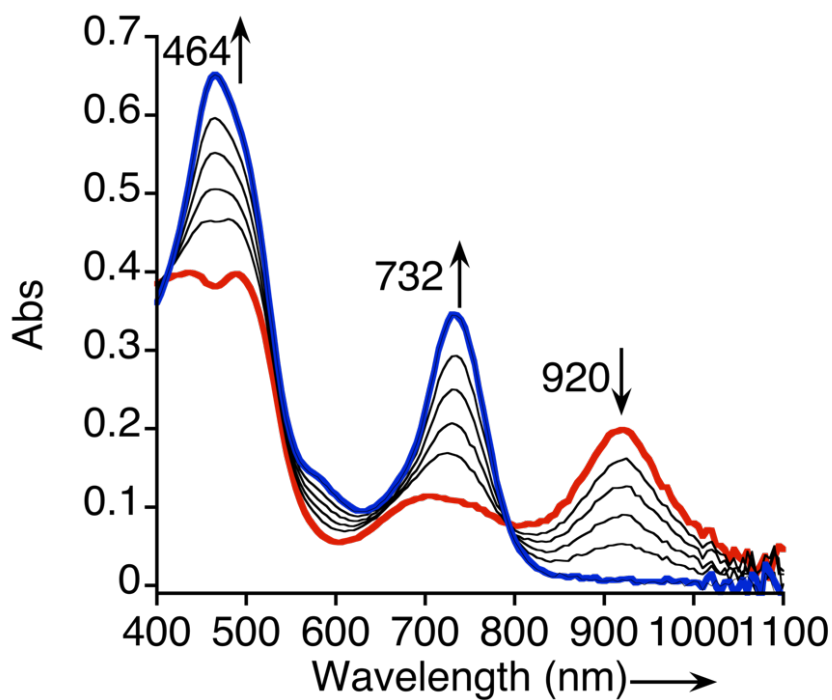
Figure S11. UV-vis spectral titration of [\text{Re}^{\text{V}}(\text{O})(\text{N-MeTBP}_8\text{Cz})]^+ ( 3 ) + [(\text{C}_5\text{H}_5)_2\text{Fe}][\text{PF}_6] (0 – 1 equiv) in \text{CH}_2\text{Cl}_2 .
