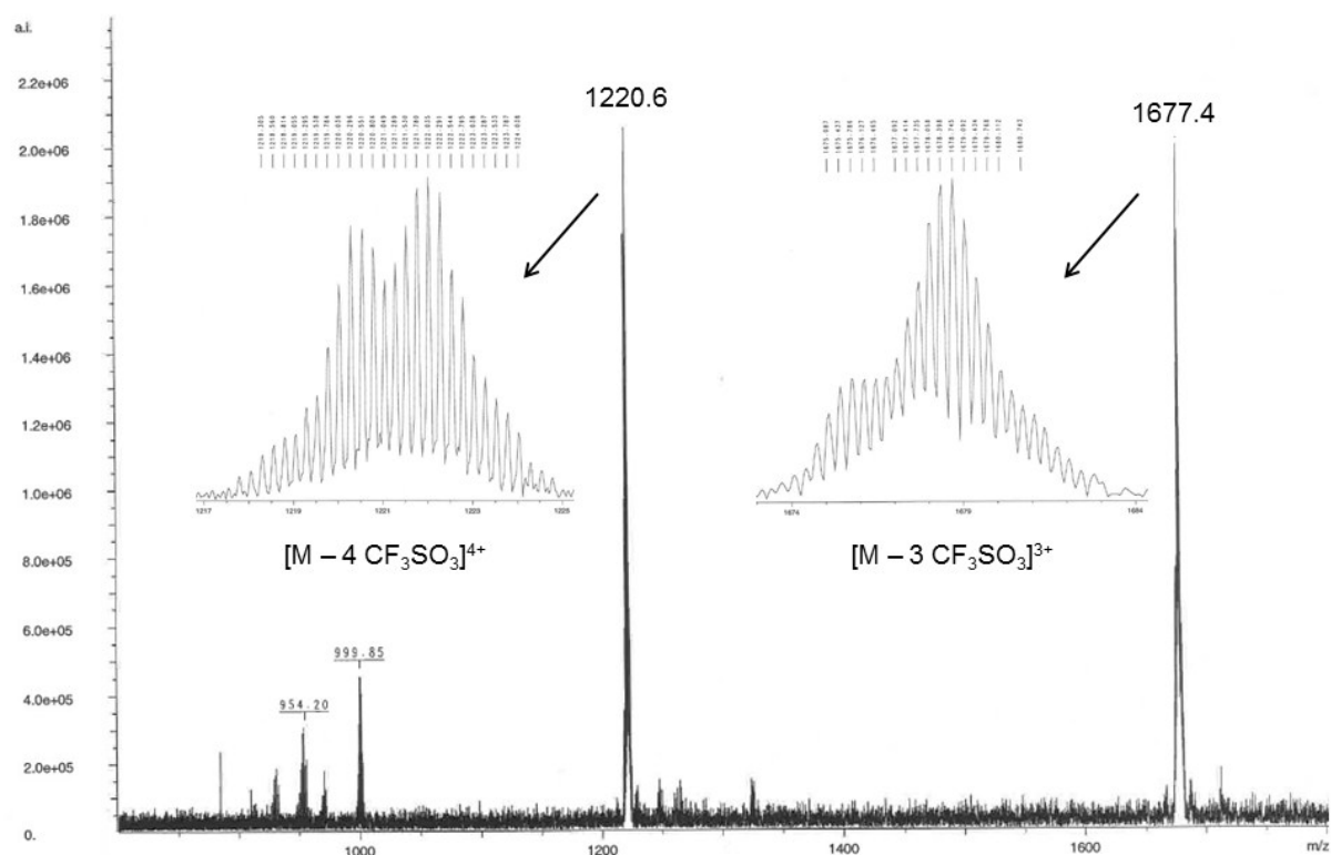
Figure S1: Electrospray ionization mass spectrum of [1][\text{CF}_3\text{SO}_3]_8 .
