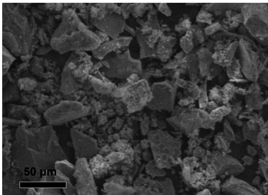
Fig. S2 SEM image of contact masses with (\text{CuO})_{19}\text{ZnO} porous hollow spheres after reaction.
